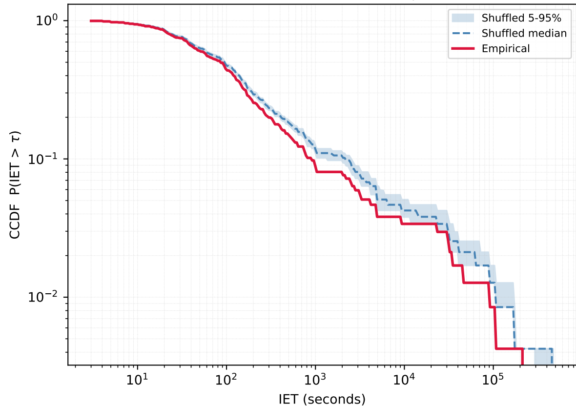
User 1095473116 - Empirical vs Reshuffled | KS=0.046 p=0.000
